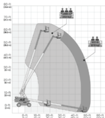
Telescopic Boom Lift JLG 600S
