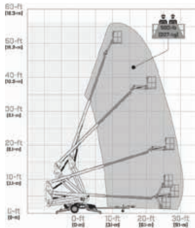
Towable Boom Lift JLG T500J
