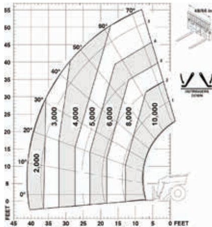
Telehandler MANITOU MTA 10055
