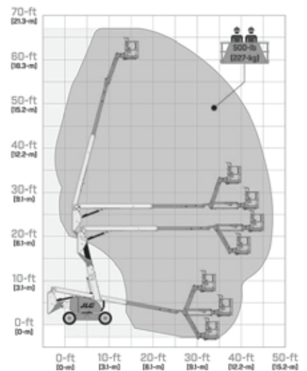
Telescopic Boom Lift JLG EC600SJ
