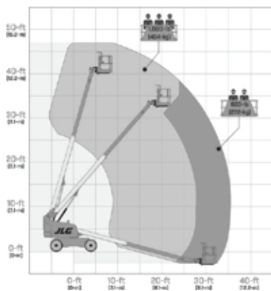
Telescopic Boom Lift JLG 400S
