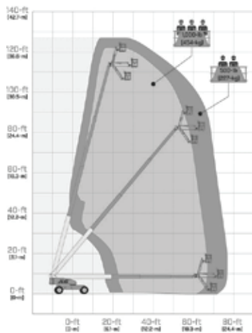
Telescopic Boom Lift JLG 1200SJ
