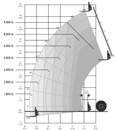
Telehandler JCB 509-42
