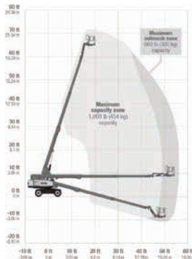
Telescopic Boom Lift GENIE S-65 XC
