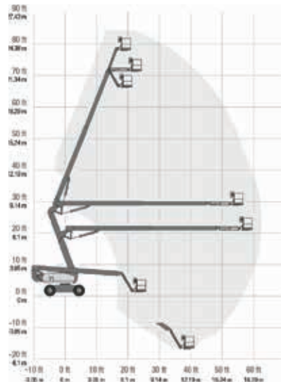
Articulating Boom Lift GENIE Z-80/60
