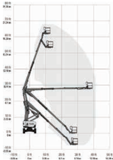
Articulating Boom Lift GENIE Z-62/40
