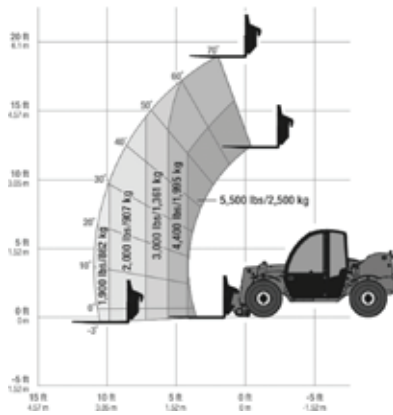
Telehandler GENIE GTH-5519
