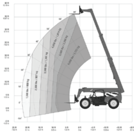
Telehandler GENIE GTH-636
